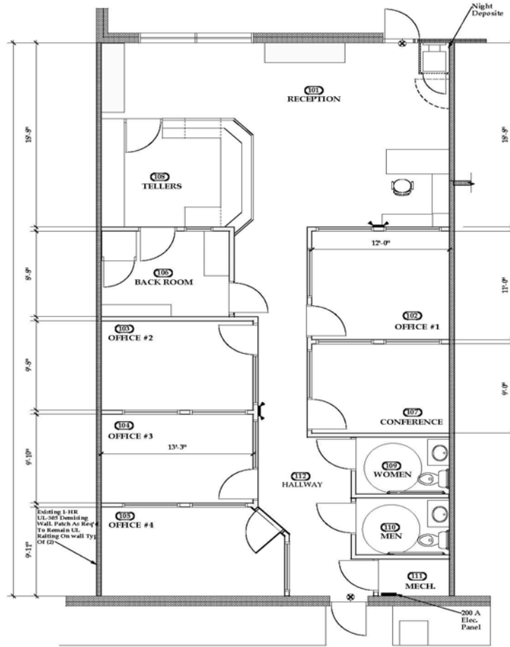
FLOOR PLAN Scale = NTS
